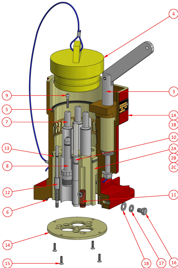
Receptacle shown fitted with "Optional" Actuator
